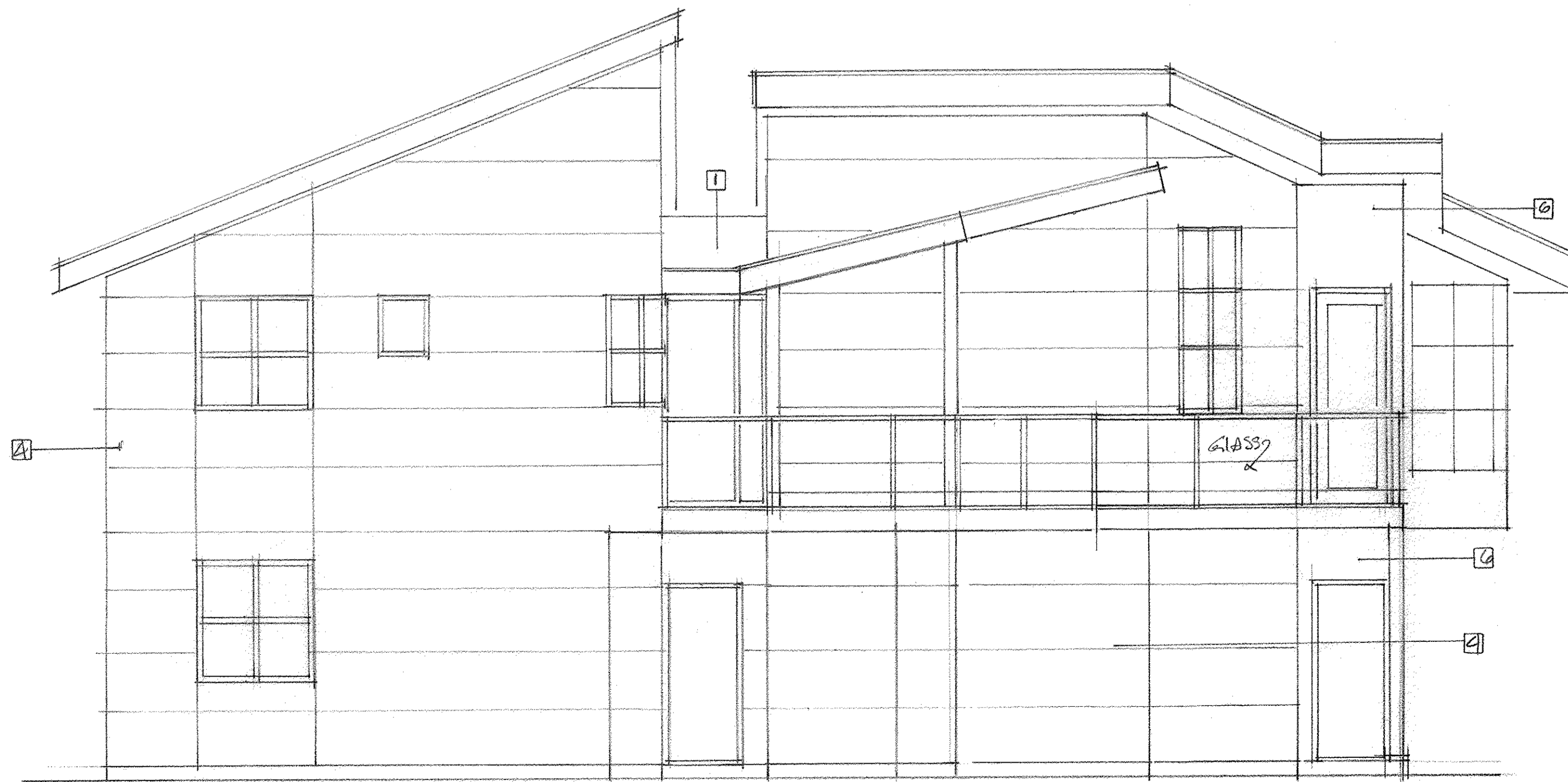
NORTH ELEVATION • 1/4" = 1'-0"
